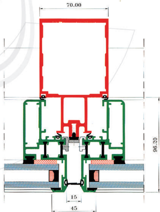
DETAIL-Q
