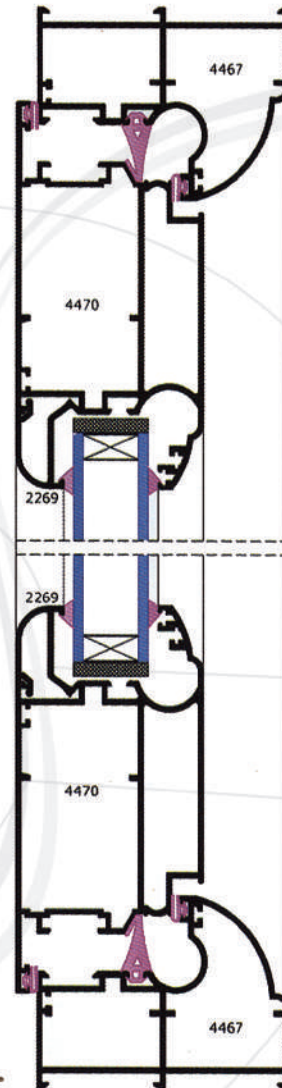
VERTICAL SECTION ( 3-4 )
