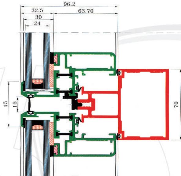
DETAIL-R
