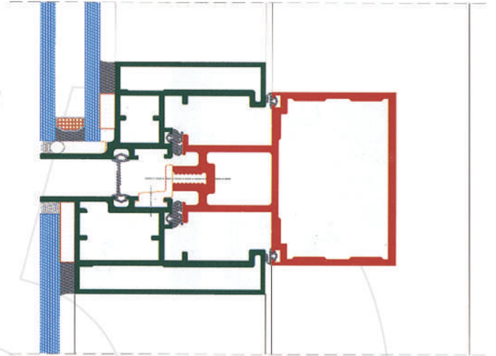
DETAIL-3
