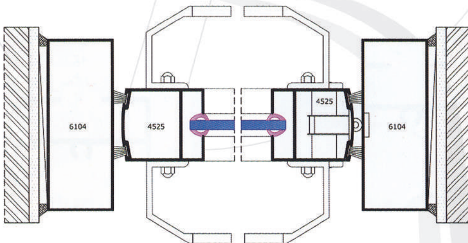
HORIZONTAL SECTION ( 1-2 )
