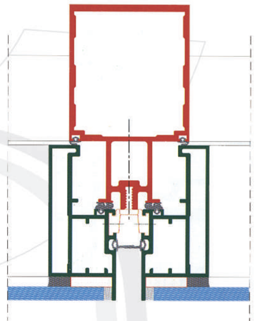
DETAIL-2
