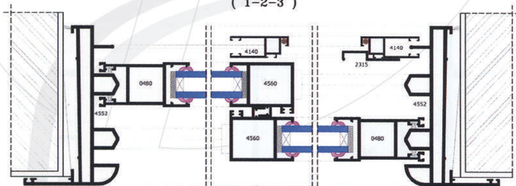
HORIZONTAL SECTION ( 1-2-3 )
