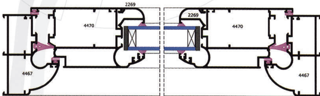
HORIZONTAL SECTION ( 1-2 )
