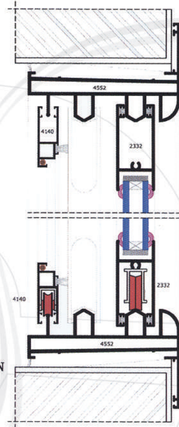
VERTICAL SECTION ( 4-5 )
