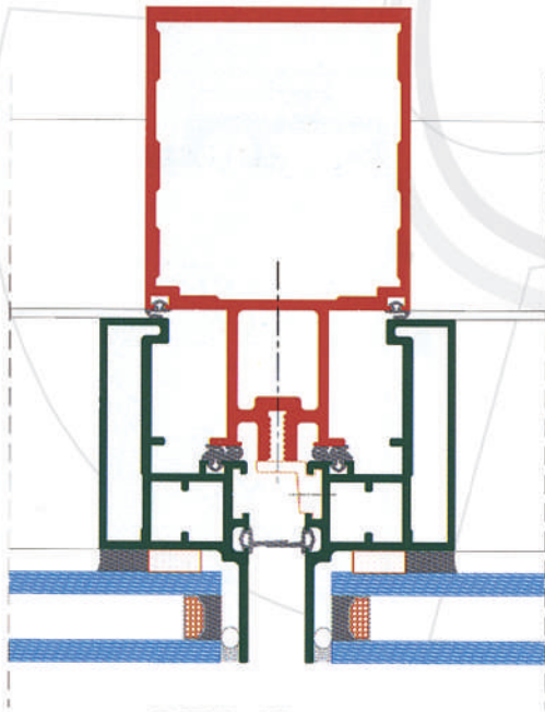
DETAIL-1
